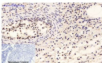
Immunohistochemical analysis of paraffin-embedded Rat-lung tissue. 1, ERK 1/2 (phospho Tyr222/205) Polyclonal Antibody was diluted at 1:200 (4°C, overnight). 2, Sodium citrate pH 6.0 was used for antibody retrieval (>98°C, 20min). 3, Secondary antibody was diluted at 1:200 (room temperature, 30min). Negative control was used by secondary antibody only.
