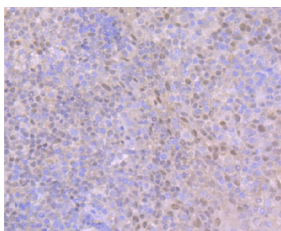
Immunohistochemical analysis of paraffin-embedded human tonsil tissue using anti-Ctip1 antibody. Counter stained with hematoxylin.
