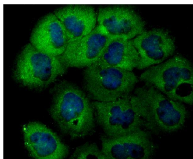
ICC staining USP14 in A431 cells (green). The nuclear counter stain is DAPI (blue). Cells were fixed in paraformaldehyde, permeabilised with 0.25% Triton X100/PBS.
