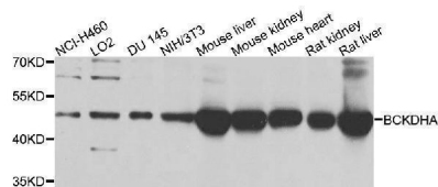
Western blotting validation for Anti-BCKDHA Antibody A04561 Western blot analysis of extracts of various cells
