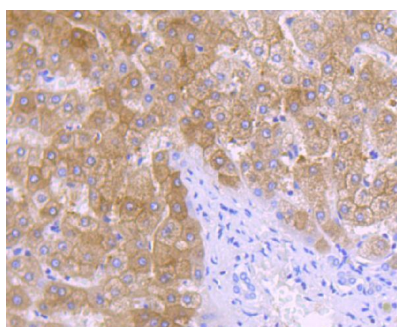
Immunohistochemical analysis of paraffin-embedded human liver tissue using anti-ALDH1L1 antibody. Counter stained with hematoxylin.
