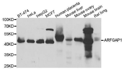
Western blot analysis of extracts of various cell lines, using ARFGAP1 antibody.
