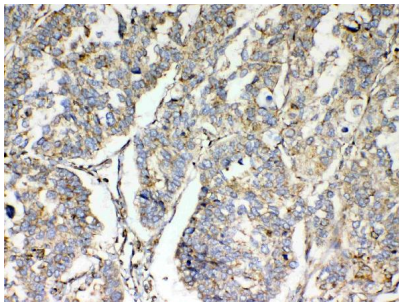
Figure 2. IHC analysis of TSPAN12 using anti-TSPAN12 antibody (A05472-1).
