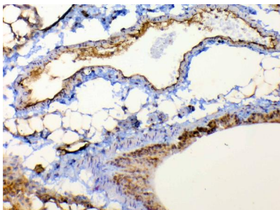
Figure 3. IHC analysis of TSPAN12 using anti-TSPAN12 antibody (A05472-1).
