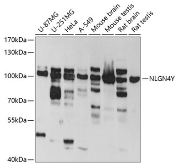
Western blot analysis of extract of various cells, using NLGN4Y antibody.
