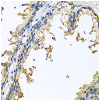
Immunohistochemistry of paraffin-embedded human prostate using NLGN4Y antibody at dilution of 1:100 (x40 lens).
