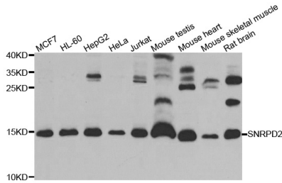
Western blot analysis of extracts of various cell lines, using SNRPD2 antibody.
