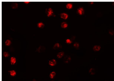
Immunofluorescence of NALP13 in K562 cells with NALP13 antibody at 20 ug/mL.
