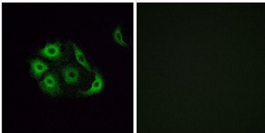
Immunofluorescence analysis of A549 cells, using OR4P4 Antibody. The picture on the right is blocked with the synthesized peptide.
