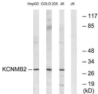
Western blot analysis of lysates from Jurkat, COLO, and HepG2 cells, using KCNMB2 Antibody. The lane on the right is blocked with the synthesized peptide.
