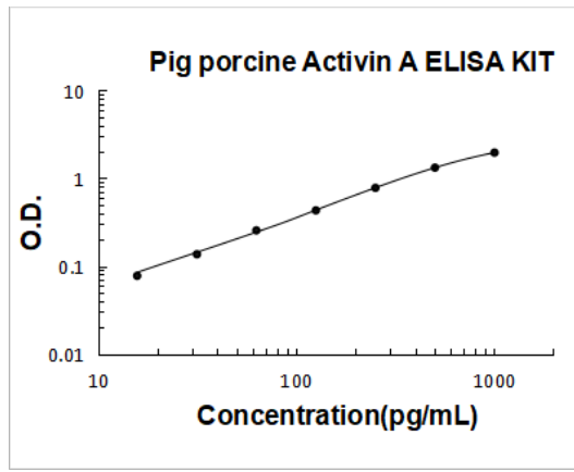
Pig Activin A PicoKine ELISA Kit standard curve
