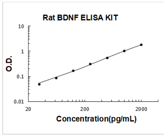
Rat BDNF PicoKine ELISA Kit standard curve
