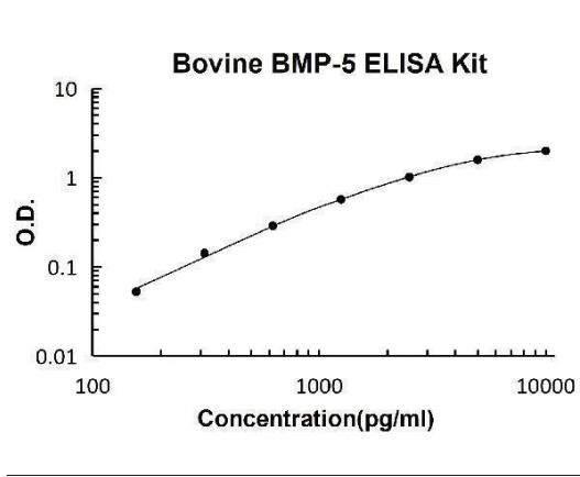
Bovine BMP-5 PicoKine ELISA Kit standard curve
