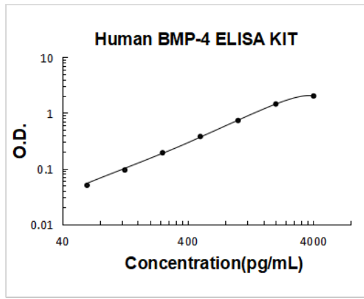
Human BMP-4 PicoKine ELISA Kit standard curve
