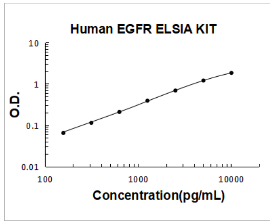
Human EGFR PicoKine ELISA Kit standard curve
