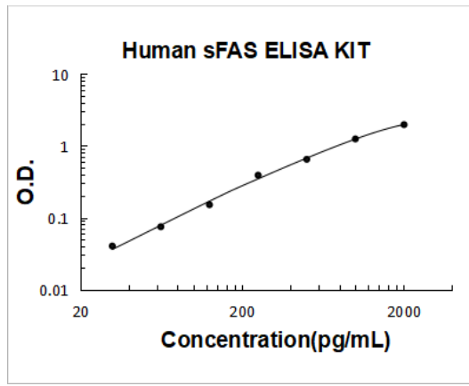
Human FAS PicoKine ELISA Kit standard curve
