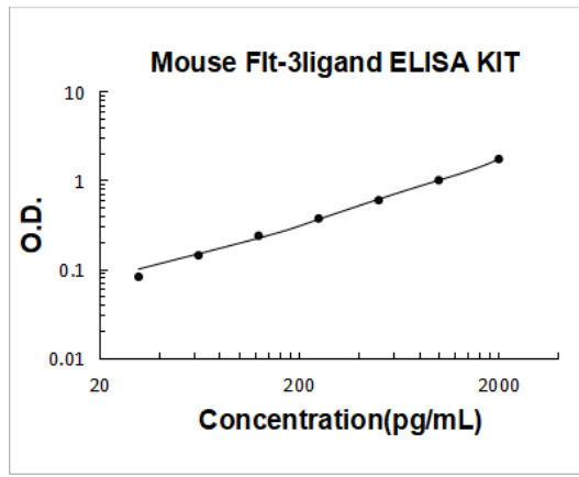
Mouse Flt-3ligand PicoKine ELISA Kit standard curve
