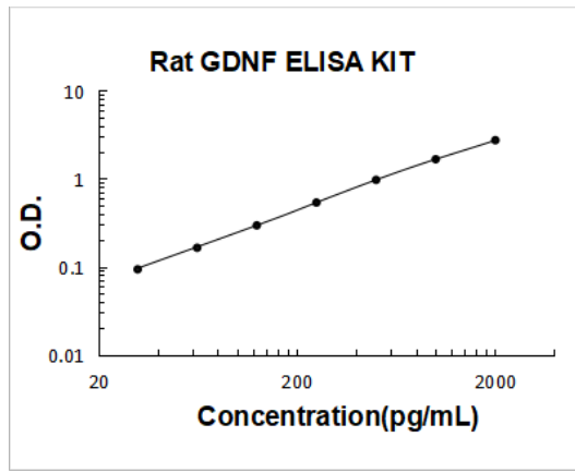
Rat GDNF PicoKine ELISA Kit standard curve
