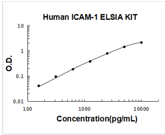
Human ICAM-1 PicoKine ELISA Kit standard curve
