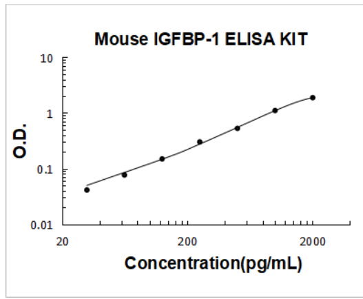
Mouse IGFBP-1 PicoKine ELISA Kit standard curve
