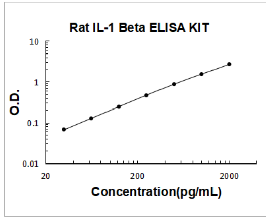
Rat IL-1 beta PicoKine ELISA Kit standard curve
