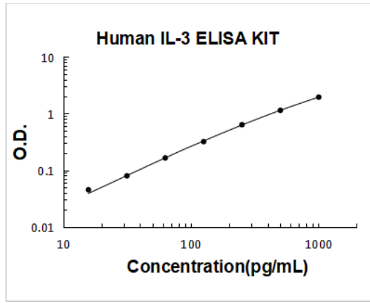
Human IL-3 PicoKine ELISA Kit standard curve
