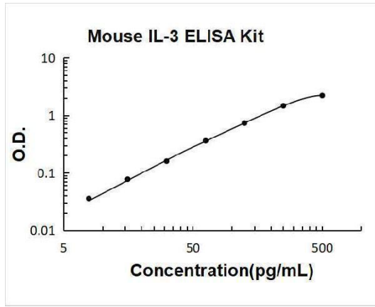
Mouse IL-3 PicoKine ELISA Kit standard curve
