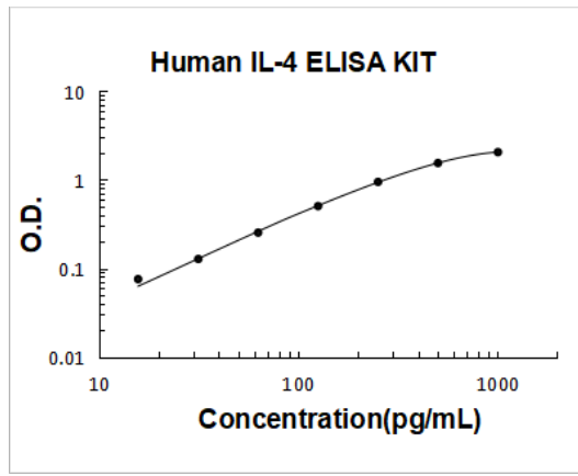
Human IL-4 PicoKine ELISA Kit standard curve
