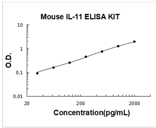
Mouse IL-11 PicoKine ELISA Kit standard curve
