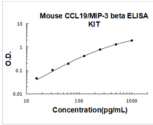
Mouse CCL19 PicoKine ELISA Kit standard curve
