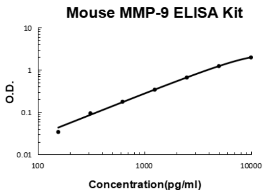
Mouse MMP-9 PicoKine ELISA Kit standard curve
