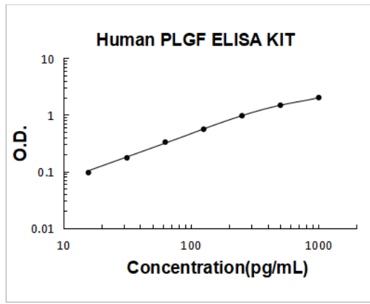
Human PLGF PicoKine ELISA Kit standard curve
