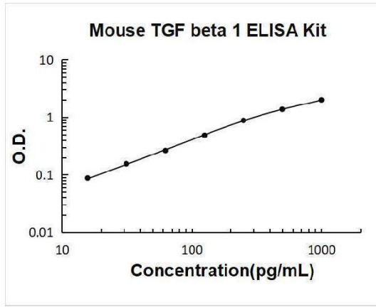
Mouse TGF beta 1 PicoKine ELISA Kit standard curve
