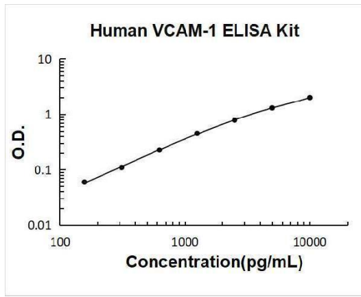
Human VCAM-1 PicoKine ELISA Kit standard curve
