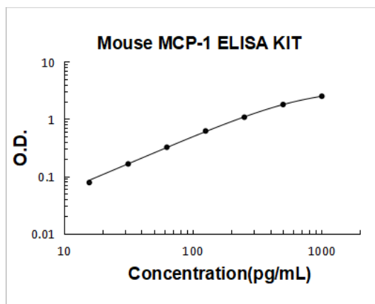
Mouse MCP-1 PicoKine ELISA Kit standard curve
