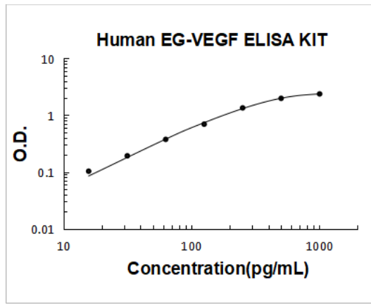
Human EG-VEGF PicoKine ELISA Kit standard curve
