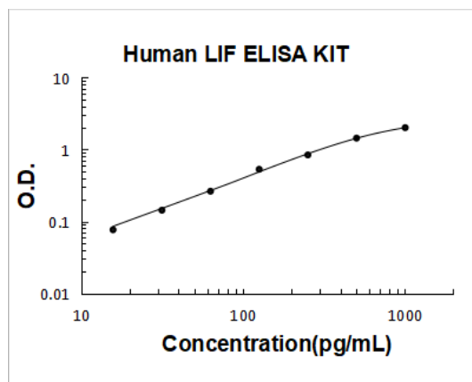
Human LIF PicoKine ELISA Kit standard curve
