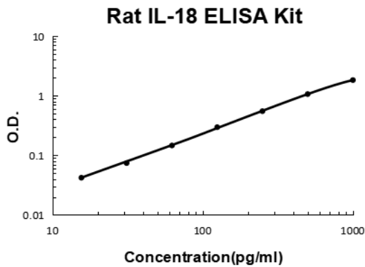
Rat IL-18 PicoKine ELISA Kit standard curve
