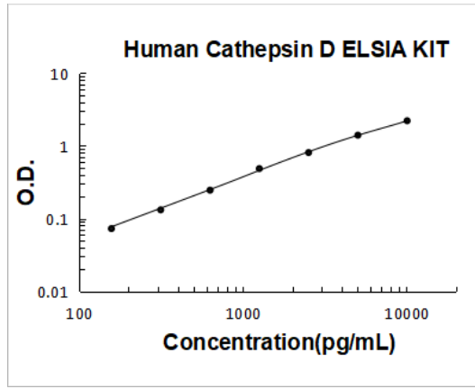
Human Cathepsin D PicoKine ELISA Kit standard curve
