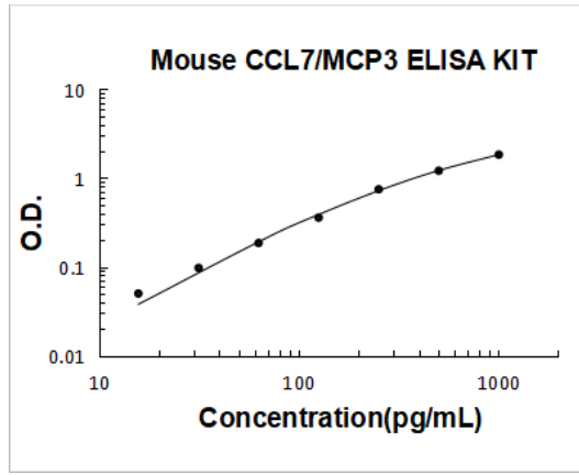
Mouse CCL7/MCP3 PicoKine ELISA Kit standard curve
