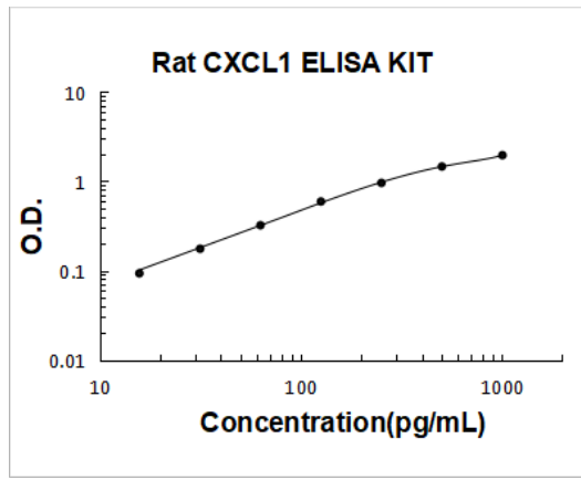
Rat CXCL1/Gro Alpha PicoKine ELISA Kit standard curve
