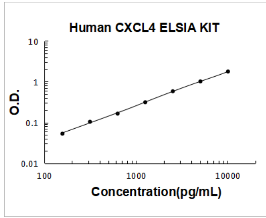
Human CXCL4/PF4 PicoKine ELISA Kit standard curve
