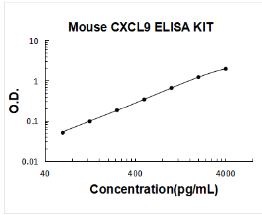
Mouse CXCL9 PicoKine ELISA Kit standard curve
