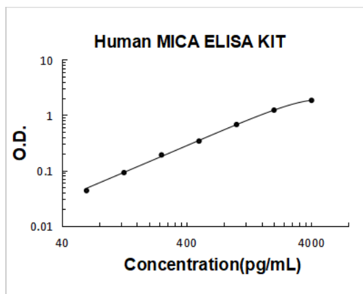
Human MICA PicoKine ELISA Kit standard curve
