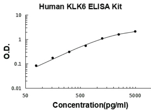
Human Kallikrein-6 PicoKine ELISA Kit standard curve
