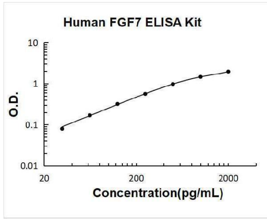
Human FGF7/KGF PicoKine ELISA Kit standard curve
