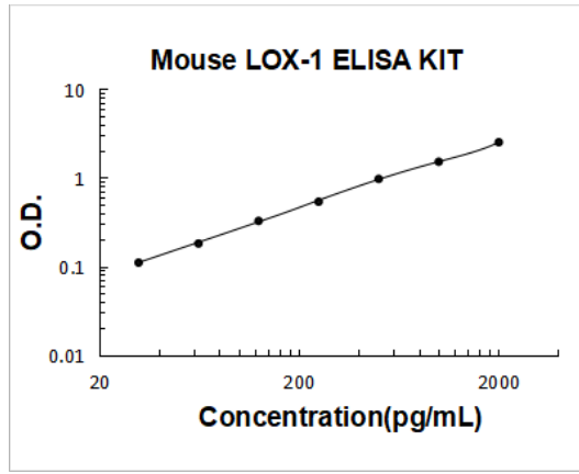
Mouse LOX-1/OLR1 PicoKine ELISA Kit standard curve
