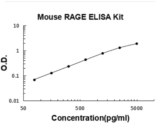
Mouse RAGE PicoKine ELISA Kit standard curve
