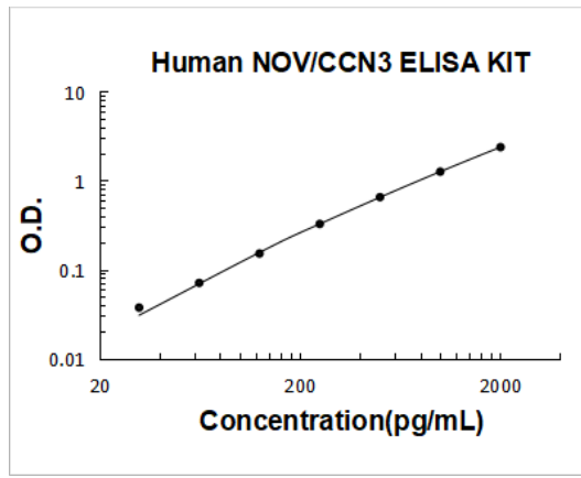
Human NOV/CCN3 PicoKine ELISA Kit standard curve
