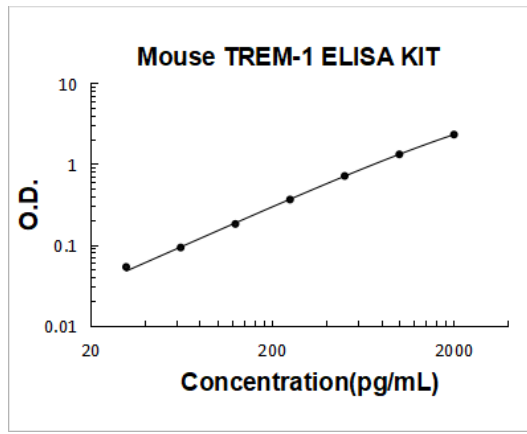
Mouse TREM-1 PicoKine ELISA Kit standard curve
