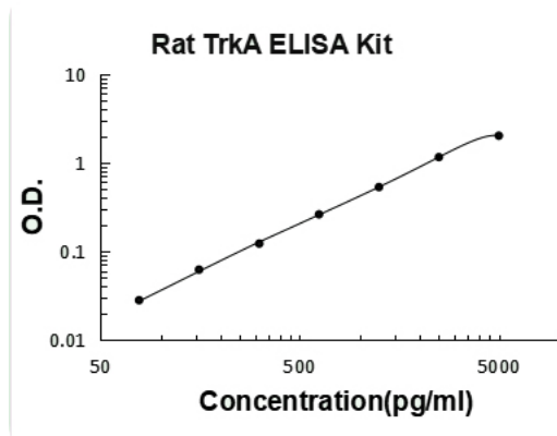
Rat TrkA PicoKine ELISA Kit standard curve
