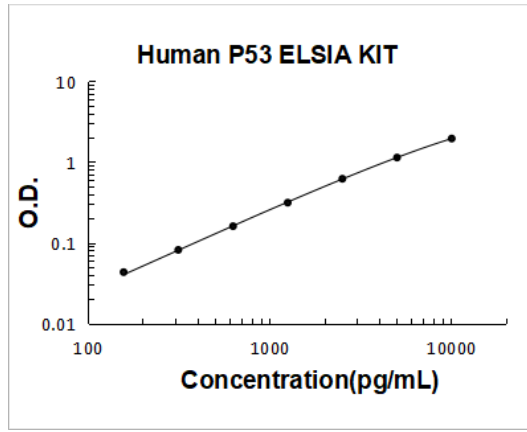
Human P53 PicoKine ELISA Kit standard curve
